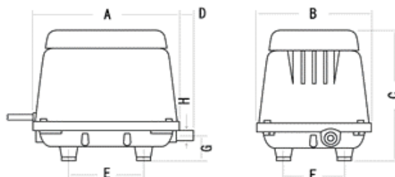
Dimensions (mm)
