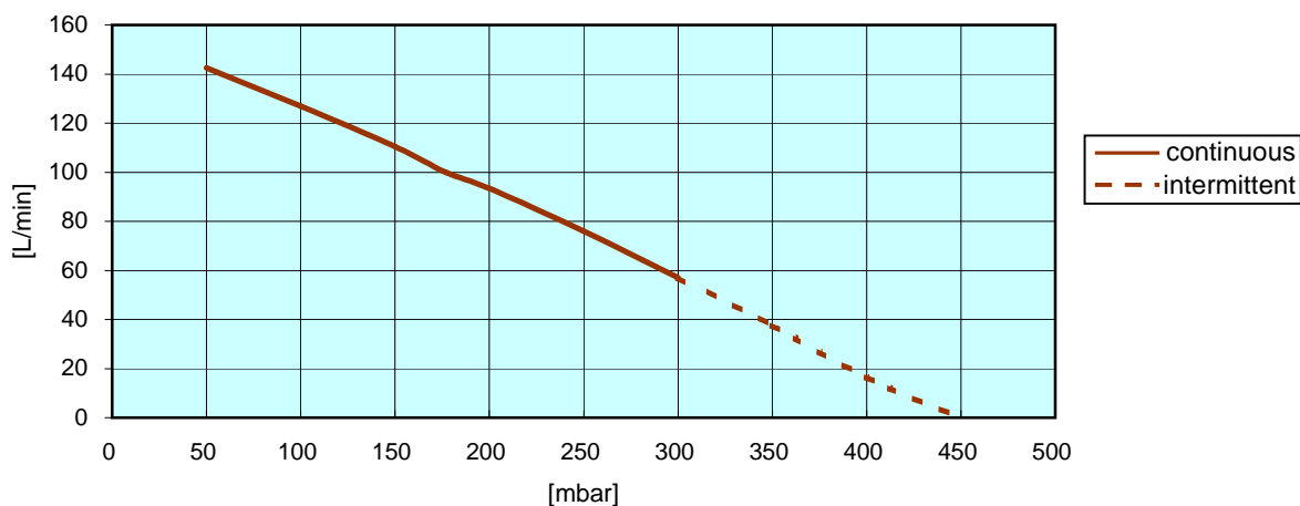
HP 100 Q-H Performance Curves
